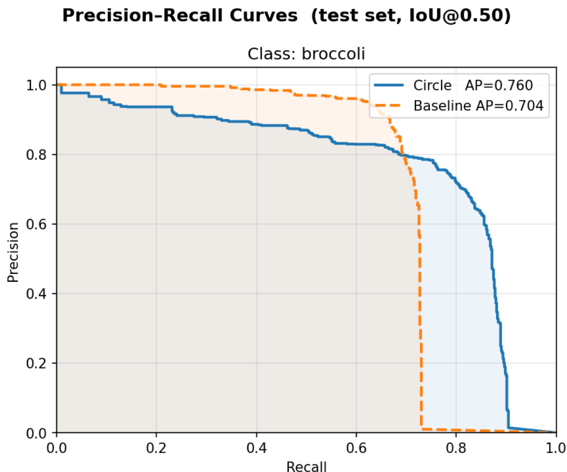
Figure 4.2: Precision-Recall curves
